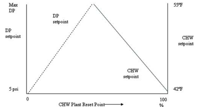
Figure 5 CHWST and DP reset.
