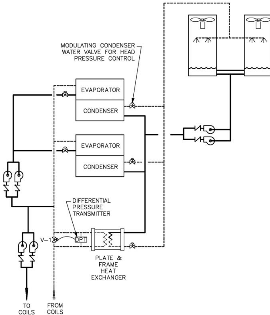
Figure 1 Integrated economizer—primary/secondary.
