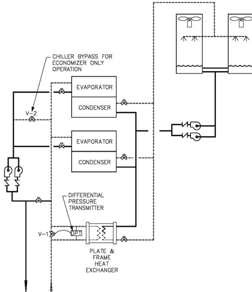
Figure 2 Integrated economizer—primary only.
