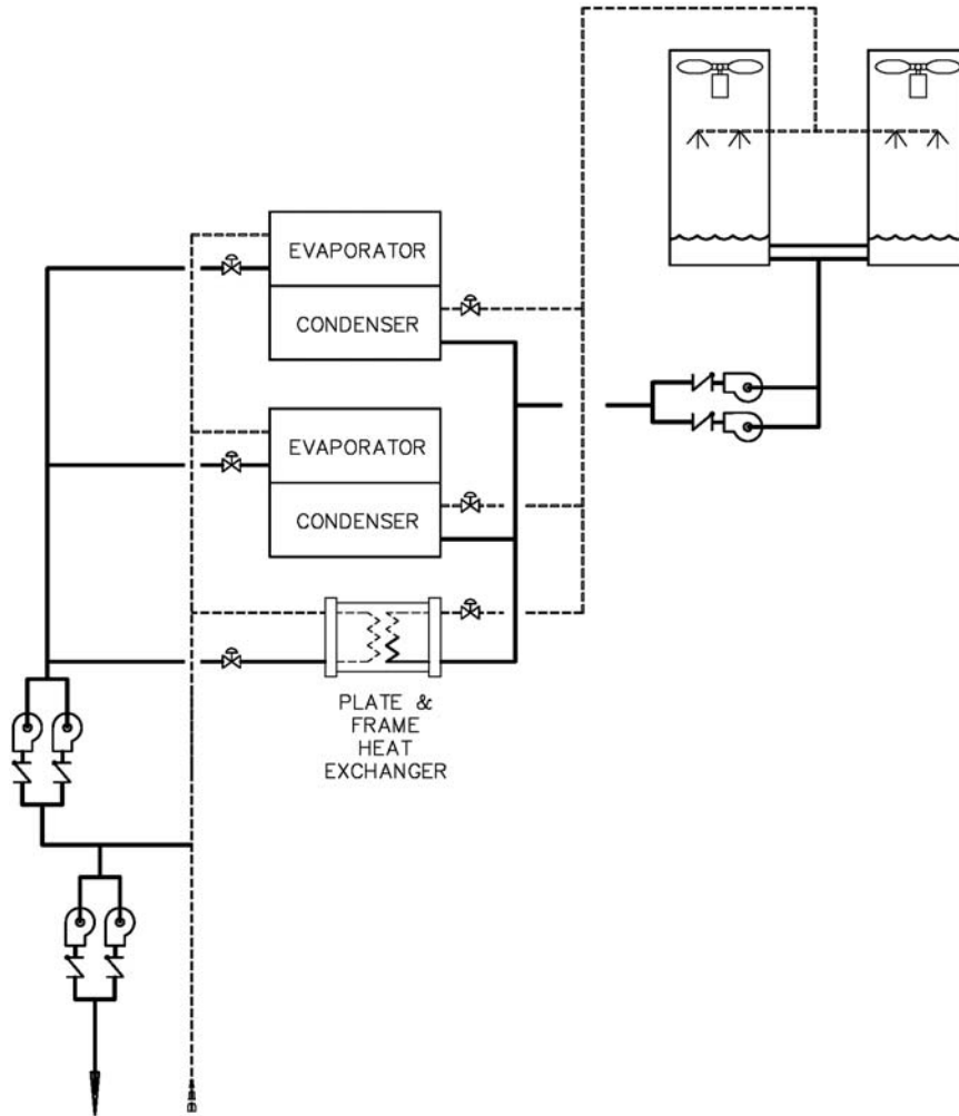
Figure 3 Non-integrated economizer.
