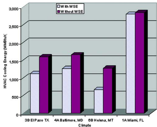
Figure 4 Waterside economizer savings in 4 climates.
