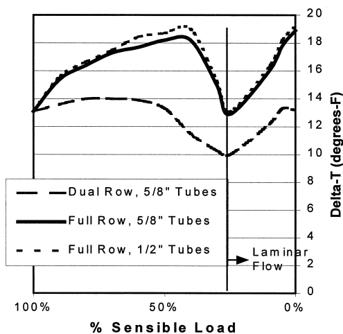
Figure 7 Delta-T at part load. Coils shown were selected for a 13°F design delta-T. Load reduction is first by reducing volume to 40%, then reducing entering air temperature. Leaving air temperature is constant, as per standard VAV systems. Performance determined by coil manufacturer’s expanded simulation program, allowing simulation below the laminar region.
