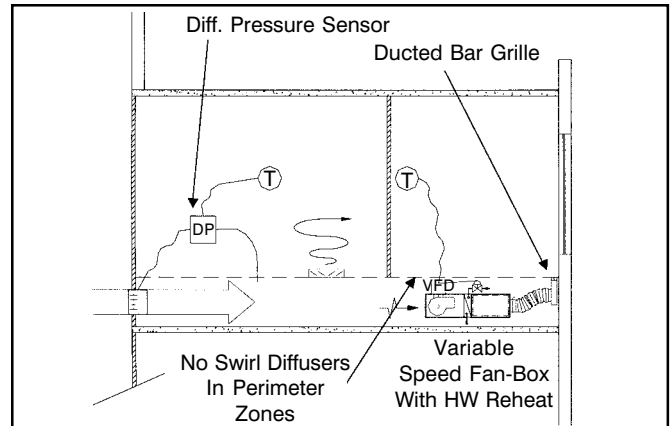
Figure 4: Cascading control loop to make a variable-volume interior zone with an independent perimeter system.
