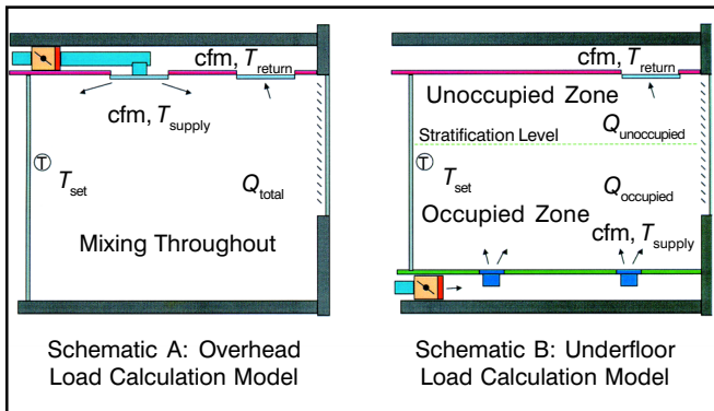
Figure 3: Load calculation models.
